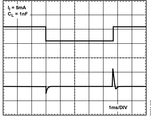
Figure 18. Load Transient
