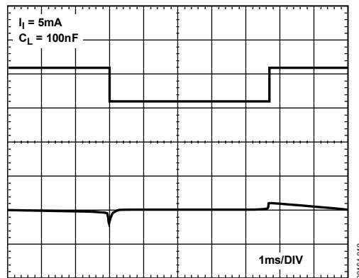
Figure 19. Load Transient
