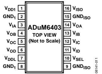
Figure 11. ADuM6403 Pin Configuration
