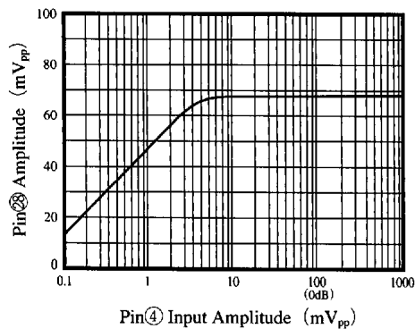
Limiter-Up Characteristics
