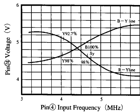
Discriminator S-Characteristics
