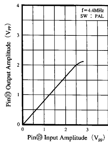
PAL Amp I/O Characteristics
