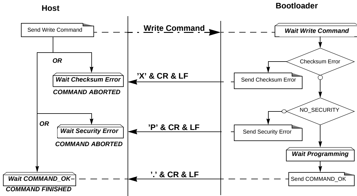
Figure 43. Write/Program Flow
