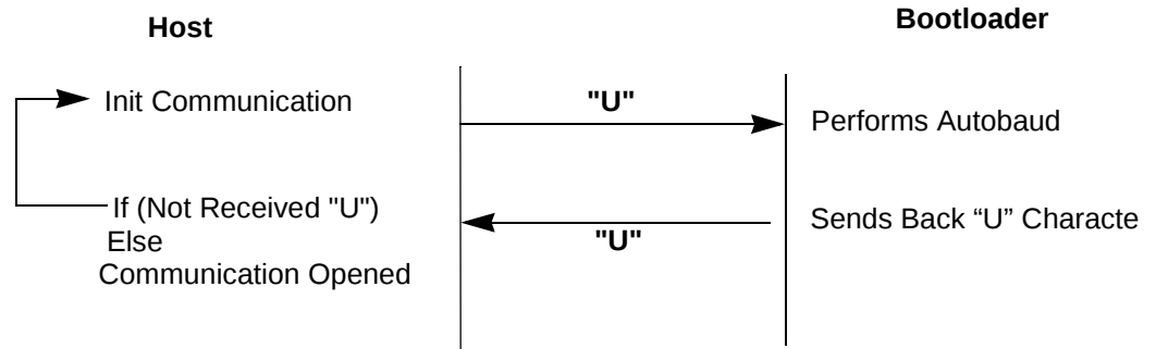
Figure 41. Initialization
