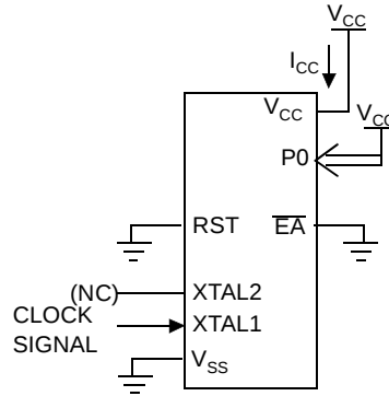
Figure 48. I_{CC} Test Condition, Idle Mode
