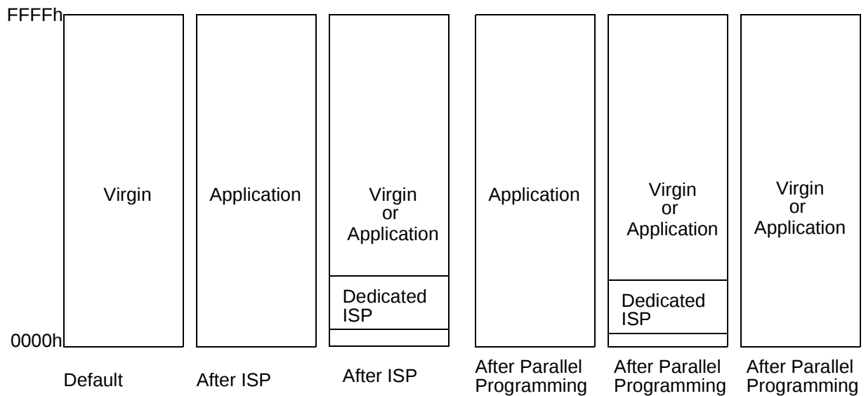
Figure 36. Flash Memory Possible Contents
