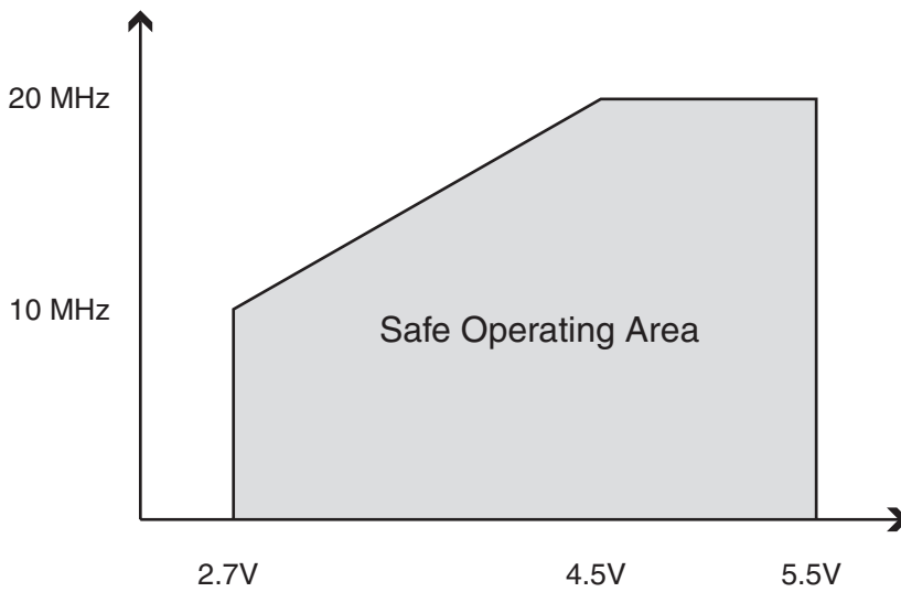
Figure 23-2. Maximum Frequency vs. V_{CC}
