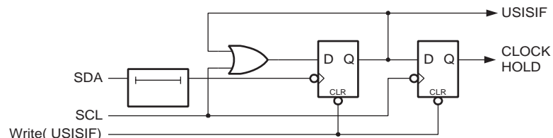
Figure 17-6. Start Condition Detector, Logic Diagram
