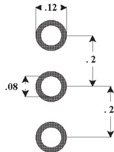
TO-247-3
