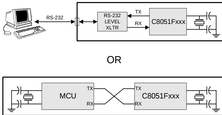
Figure 21.6. UART0 Modes 1, 2, and 3 Interconnect Diagram
