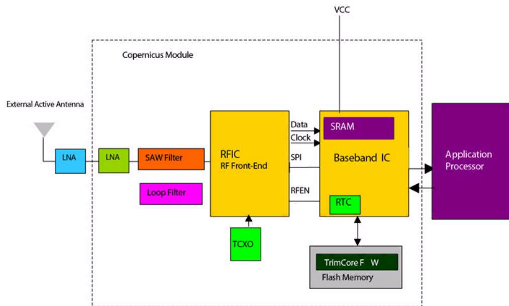
Figure 2.1 Copernicus GPS Block Diagram
