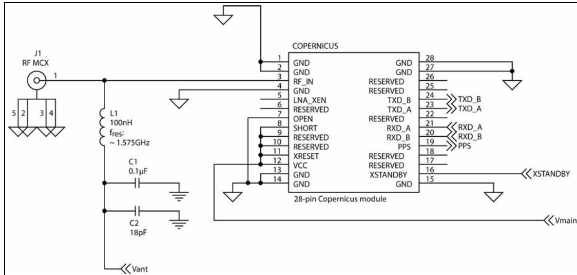
Figure 5.4 Active antenna - No Antenna Status
