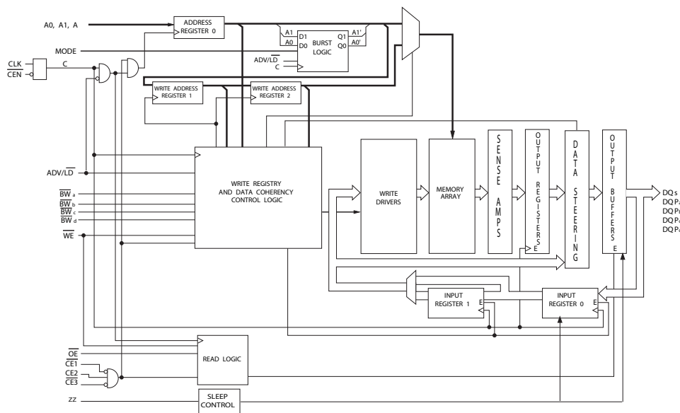
Logic Block Diagram-CY7C1370D (512K x 36)
