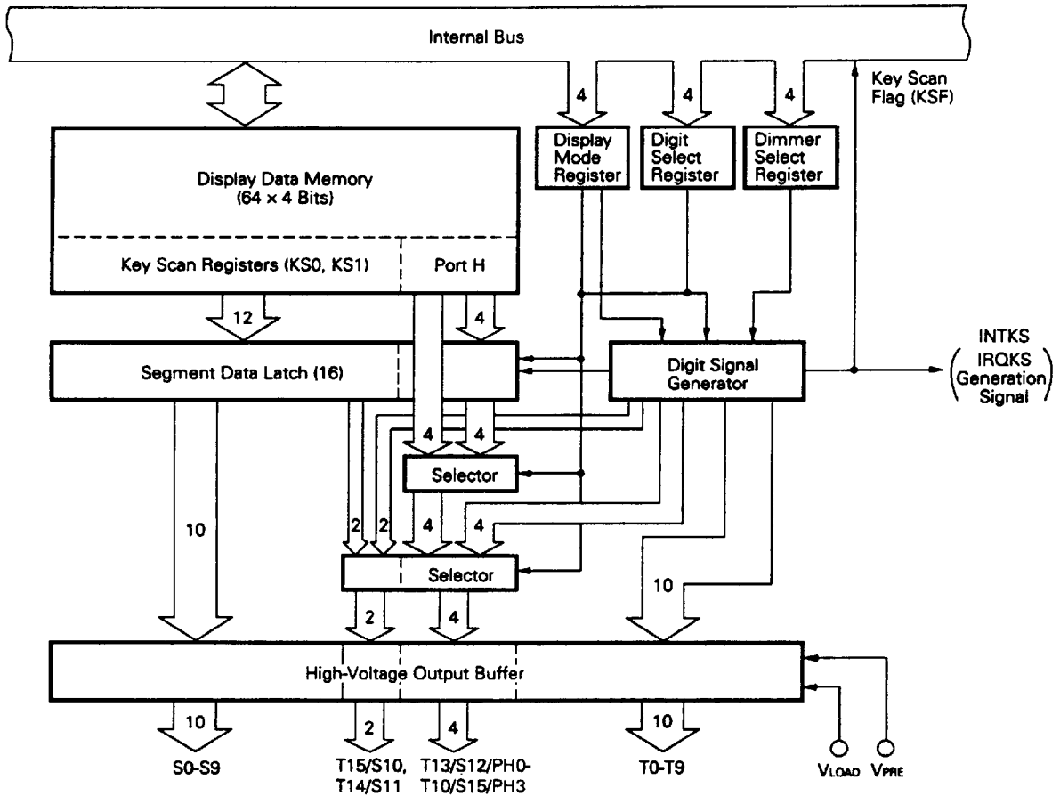
Fig. 5-8 FIP Controller/Driver Block Diagram
