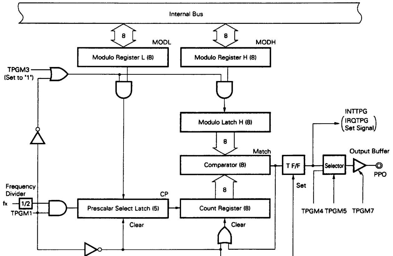
Fig. 5-5 Block Diagram of Timer/Pulse Generator (Timer Mode)
