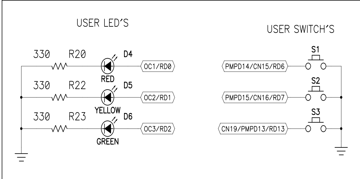
FIGURE A-5: PIC32MX SCHEMATIC, SHEET 5 OF 6 (SWITCHES AND LEDES)
