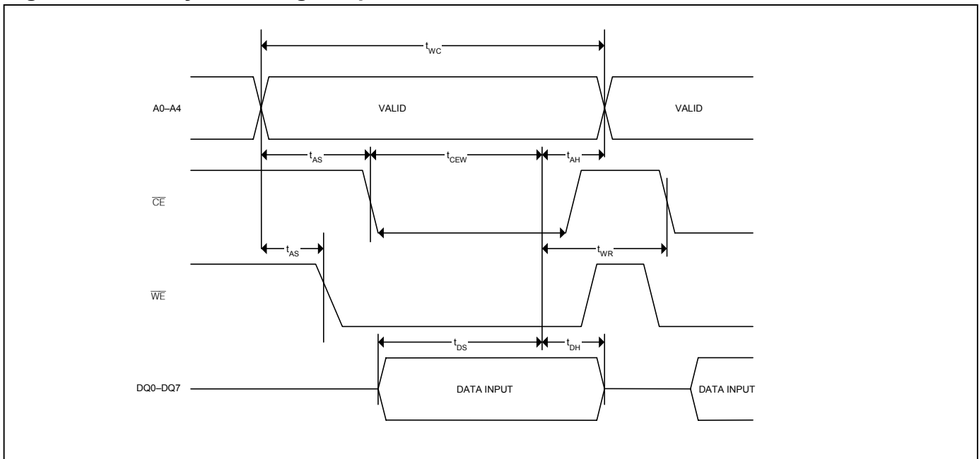
Figure 3. Write Cycle Timing, Chip-Enable-Controlled
