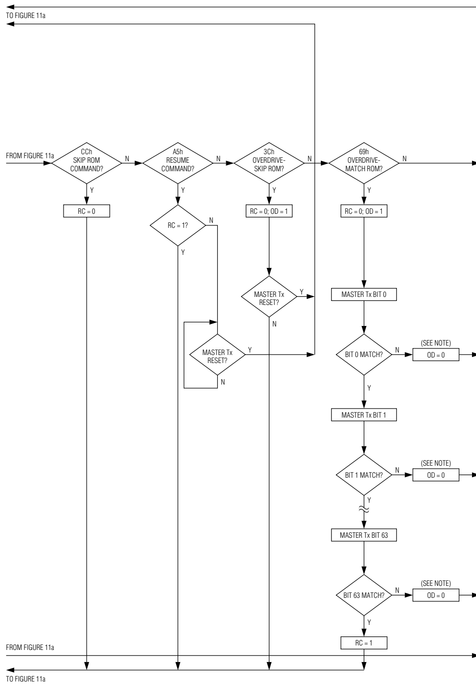
Figure 11b. ROM Functions Flowchart (continued)
