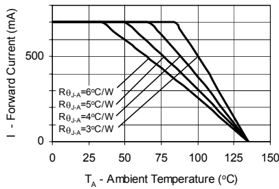
Figure 5a. Maximum Forward Current vs. Ambient Temperature. Derating based on T_{JMAX} = 135^\circ\text{C} for White, Green, Cyan and Blue 12-Up.
