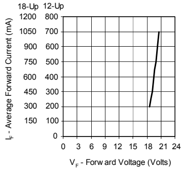
Figure 3a. Forward Current vs. Forward Voltage for White, Green, Cyan and Blue.
