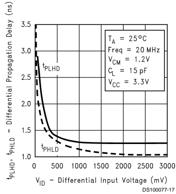
Differential Propagation Delay vs Differential Input Voltage
