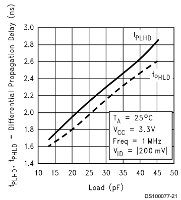
Differential Propagation Delay vs Load
