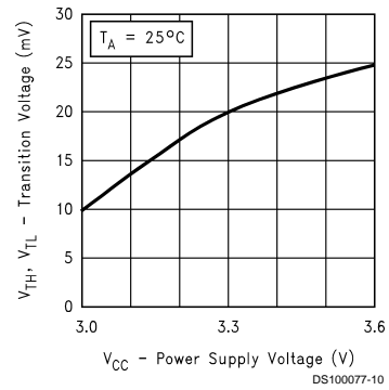
Differential Transition Voltage vs Power Supply Voltage
