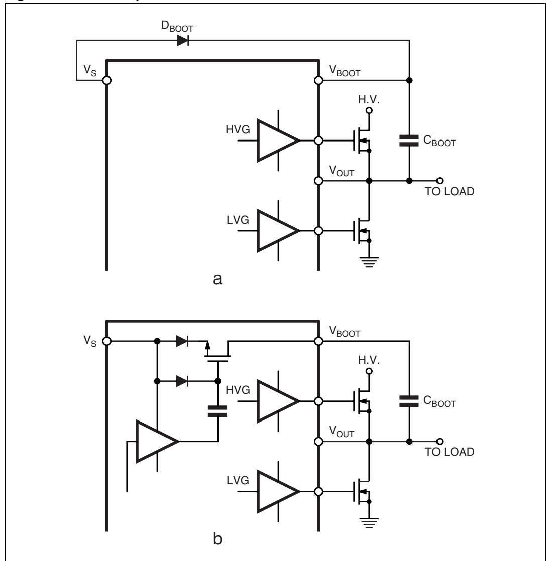
Figure 5. Bootstrap driver
