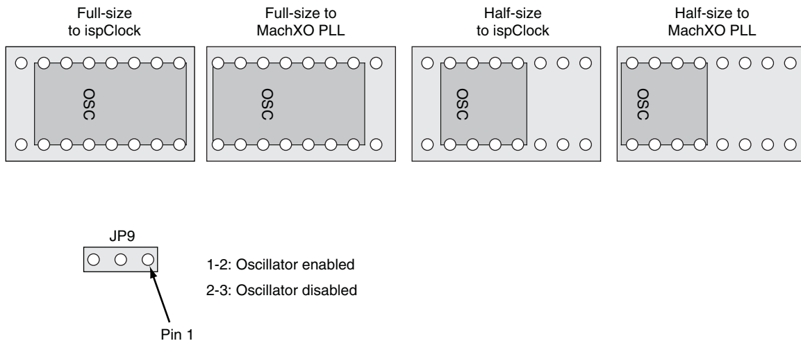
Figure 6. Oscillator Positions
