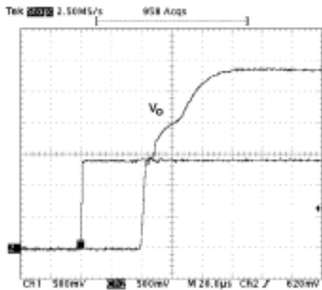
Figure 21: START-UP
