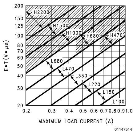
FIGURE 7. LM2575(HV)-ADJ
