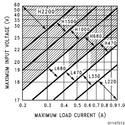
FIGURE 6. LM2575(HV)-15
