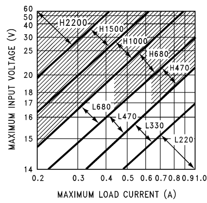
FIGURE 5. LM2575(HV)-12
