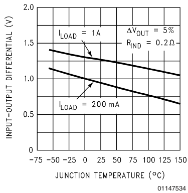
Dropout Voltage
