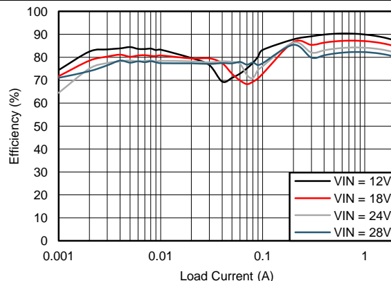
Figure 66. Efficiency
