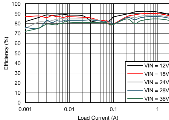
Figure 54. Efficiency
