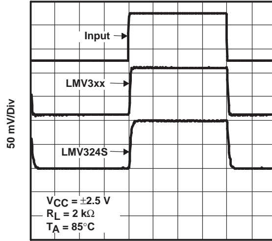
1 \mu\text{s/Div} Figure 31
