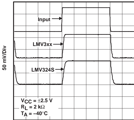
1 \mu\text{s/Div} Figure 32
