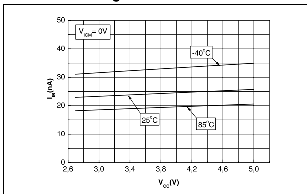
Figure 5. Input bias current versus supply voltage
