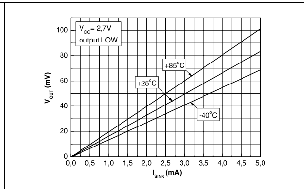
Figure 4. Output voltage versus output current at 2.7 V supply
