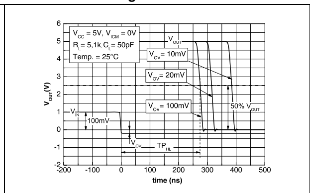
Figure 6. Response time versus overdrive with negative transition
