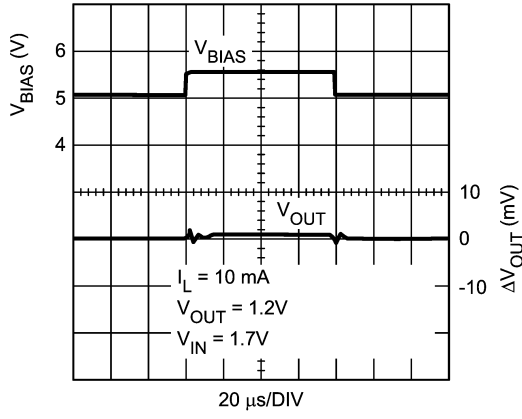
V_{BIAS} Transient Response
