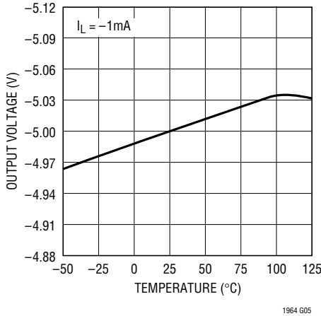
LT1964-5 Output Voltage
