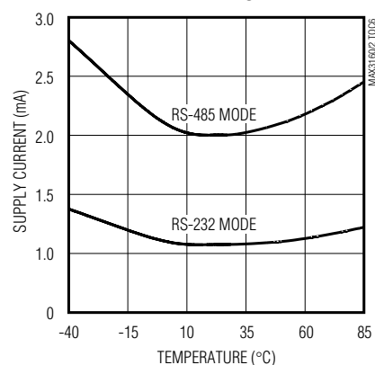
MAX3160/MAX3161 NO-LOAD SUPPLY CURRENT vs. TEMPERATURE
