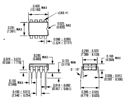
8 Lead Cerdip (JA) \theta_{JA} = 125^{\circ}\text{C/W} \theta_{JC} = 55^{\circ}\text{C/W}
