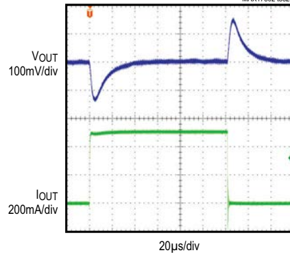
LOAD TRANSIENT RESPONSE OF MAX17502F (LOAD CURRENT STEPPED FROM NO-LOAD TO 500mA)
