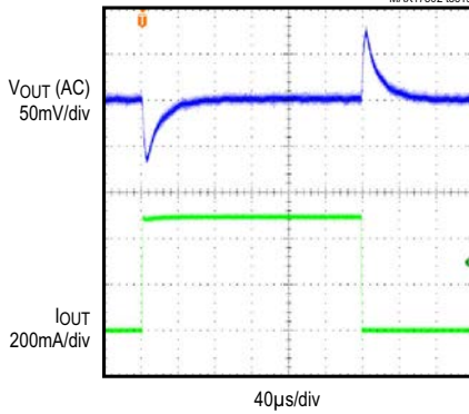
LOAD TRANSIENT RESPONSE OF MAX17502E (LOAD CURRENT STEPPED FROM NO-LOAD TO 500mA)
