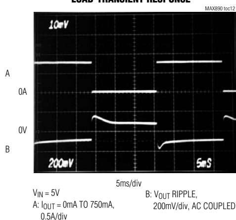
LOAD-TRANSIENT RESPONSE
