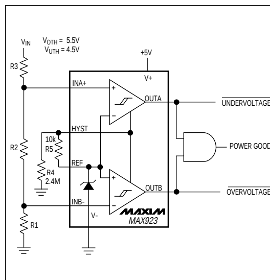
Figure 6. Window Detector
