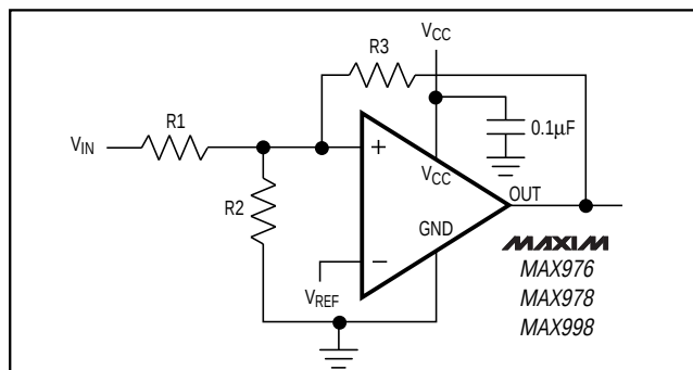
Figure 2. Additional Hysteresis
