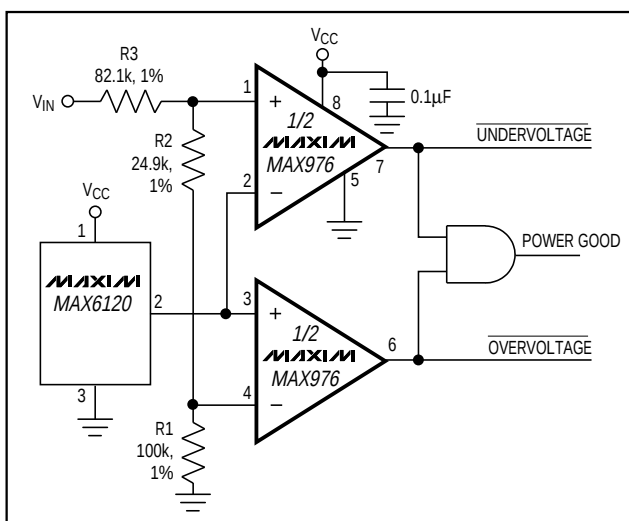
Figure 3. Window Comparator
