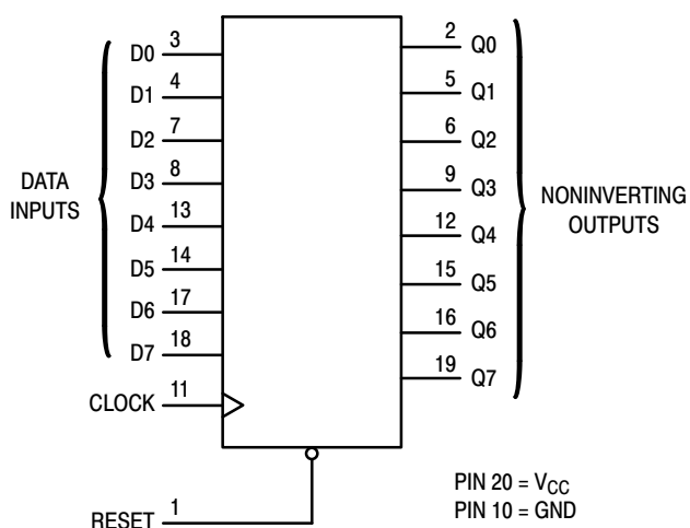
Figure 1. Logic Diagram
