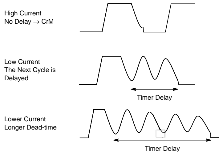
Figure 60. CCFF Operation
