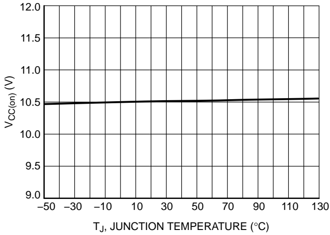
Figure 4. Start-up Threshold, V CC Increasing (V CC(on) ) vs. Temperature (A and A1 Versions)
