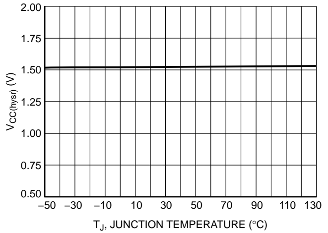
Figure 7. Hysteresis (V CC(on) - V CC(off) ) vs. Temperature (A and A1 Versions)
