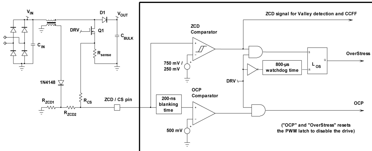
Figure 70. Current Sense and Zero Current Detection Blocks
