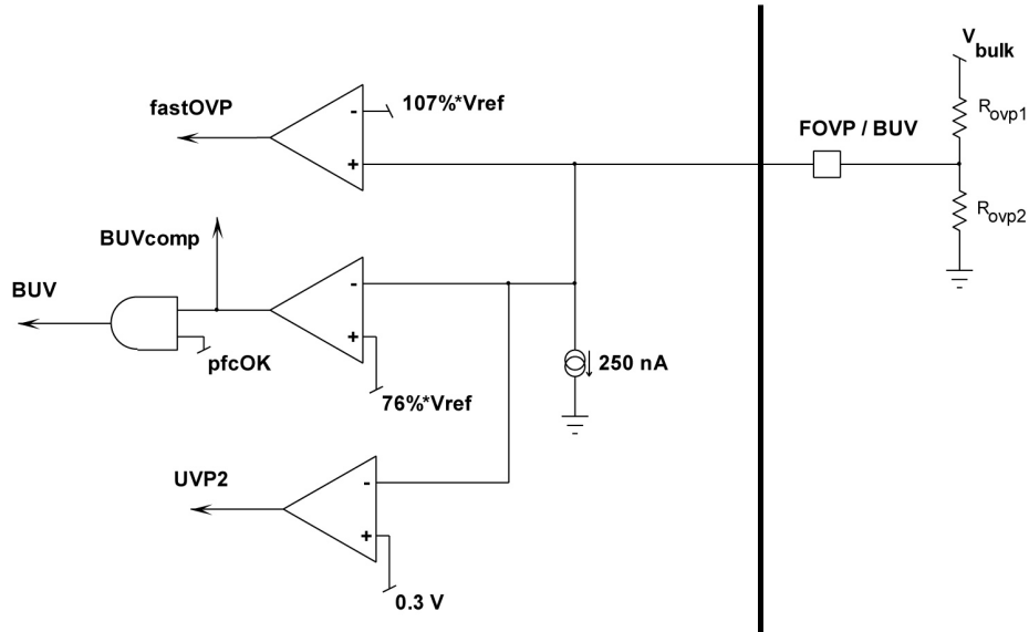
Figure 69. Bulk Under-voltage Detection (NCP1612A and NCP1612B)
