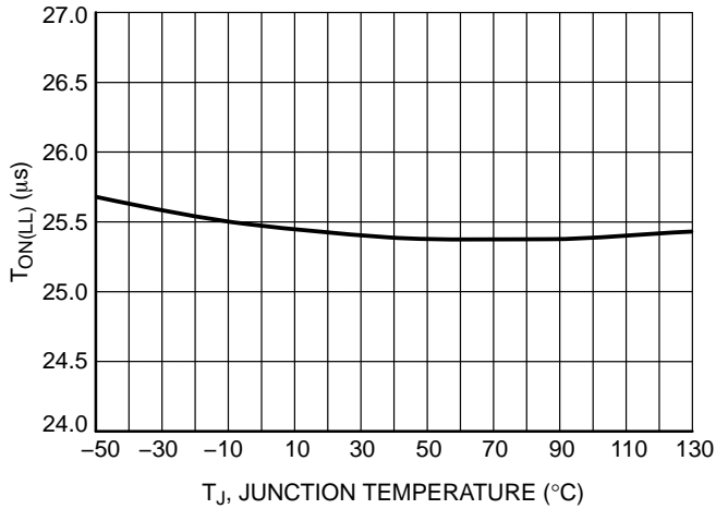
Figure 40. Maximum On Time @ V_{SENSE} = 1.4 V vs. Temperature
