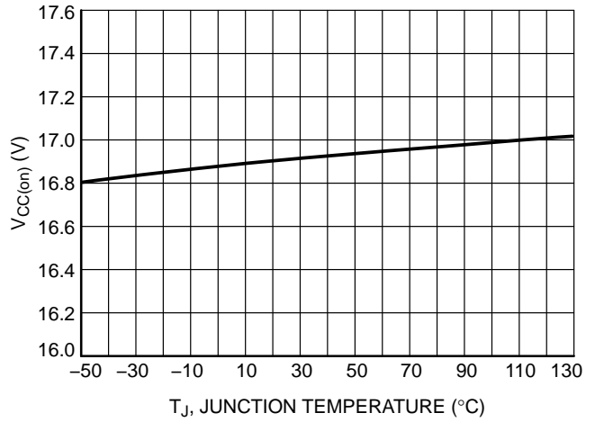
Figure 5. Start-up Threshold, V CC Increasing (V CC(on) ) vs. Temperature (B Version)
