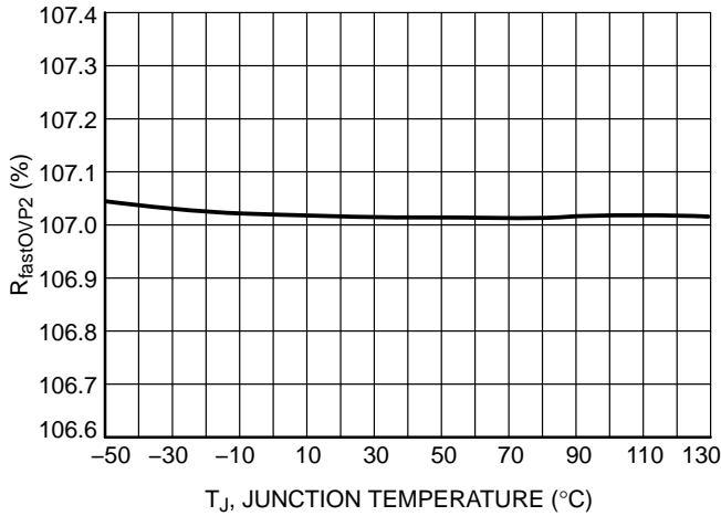
Figure 46. Ratio (fastOVP Threshold, VFOVP/BUV Rising) over VREF vs. Temperature
