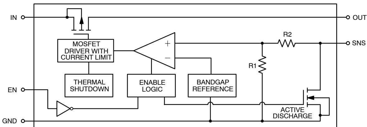
Figure 6. NCP691 Block Diagram (Fixed Version)
