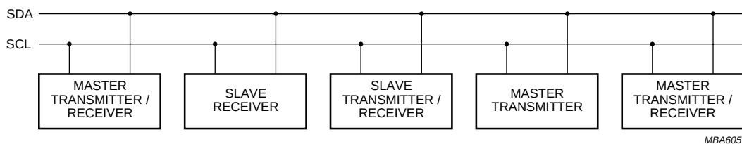
Fig 10. System configuration.
