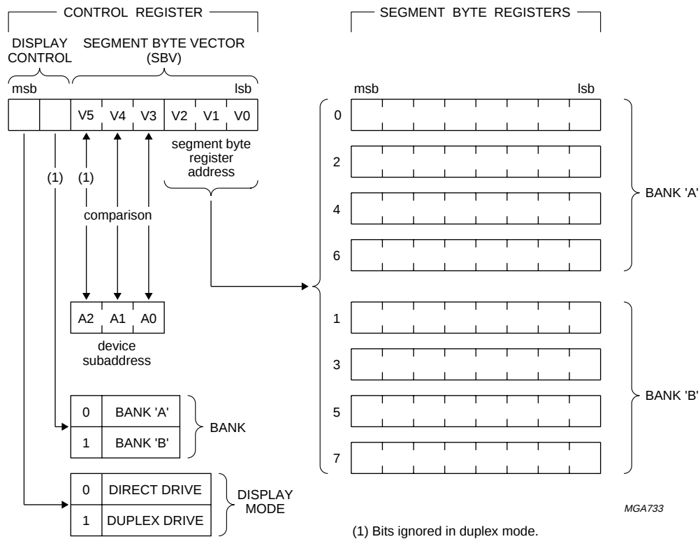
Fig.3 PCF8577C register organization.
