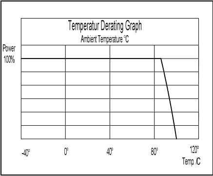
Derating Graph
