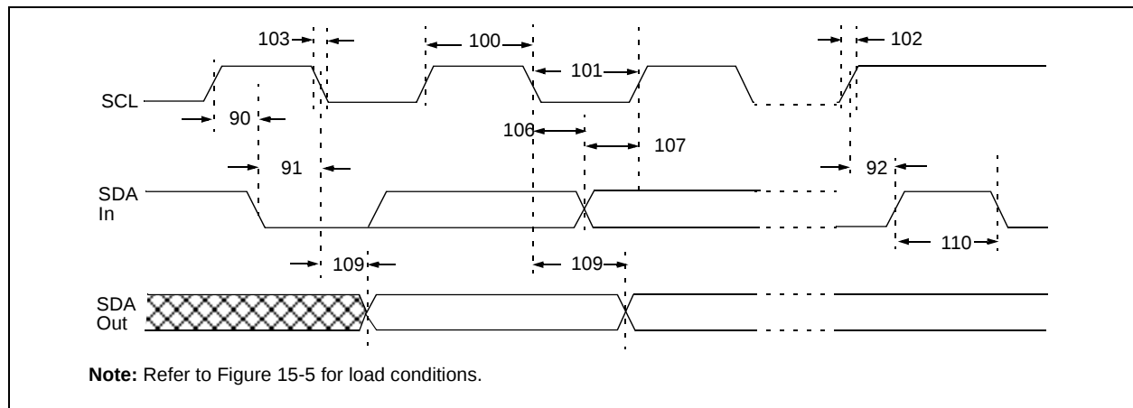
FIGURE 15-18: I 2 C BUS DATA TIMING
