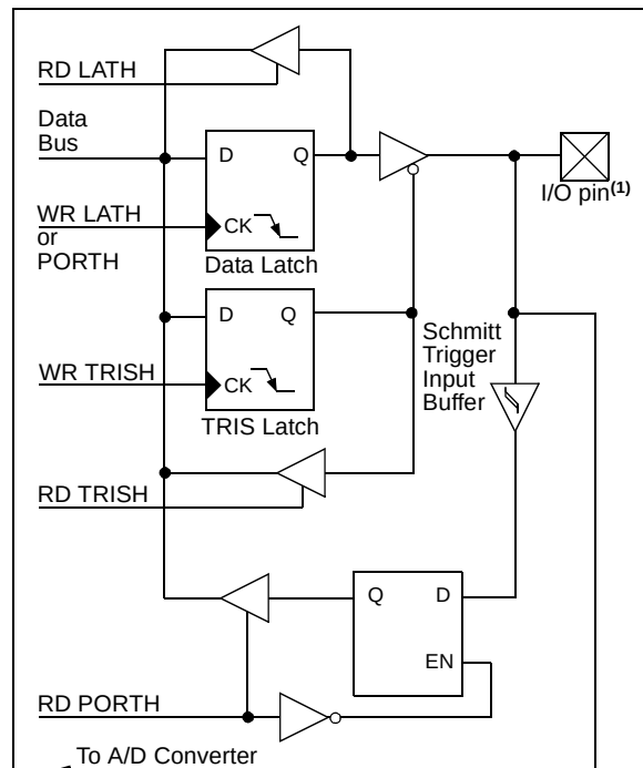
FIGURE 10-19: RH7:RH4 PINS BLOCK DIAGRAM IN I/O MODE
