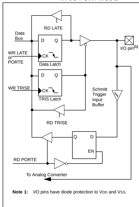
FIGURE 9-9: PORTE BLOCK DIAGRAM IN I/O PORT MODE
