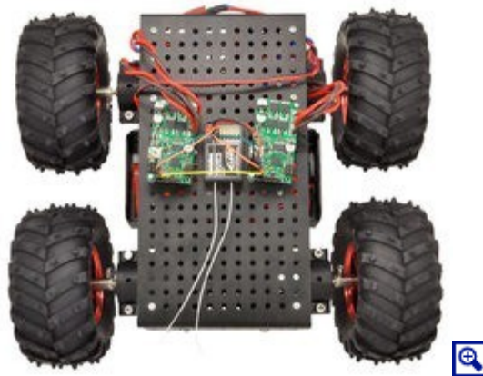
Two Pololu Simple Motor Controllers enable mixed RC-control of Dagu Wild Thumper 4WD all-terrain chassis.
