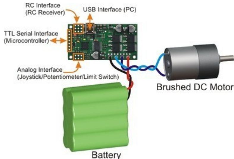
Simple High-Power Motor Controller 18v25 or 24v23 simplified connection diagram. Key Features
