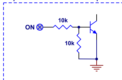
Input structure of ON input
