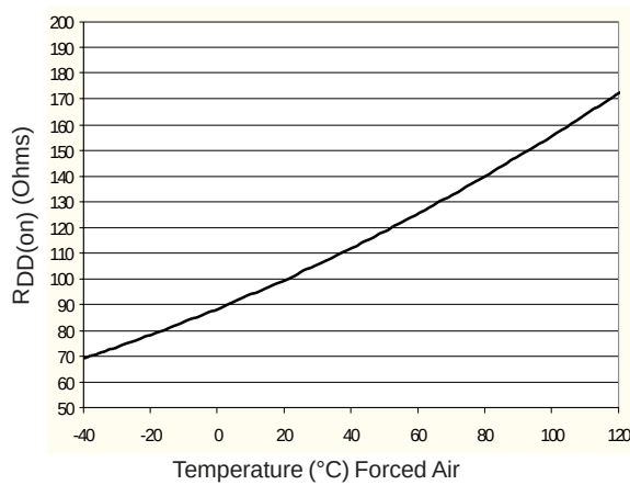
Figure 3. Typical On-Resistance
