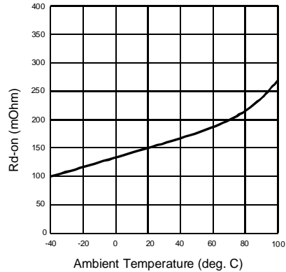
Figure 4. Typical On-Resistance
