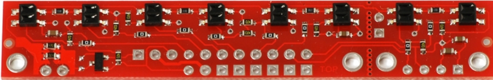
QTR-8A reflectance sensor array.
