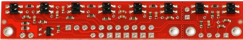
QTR-8RC reflectance sensor array.
