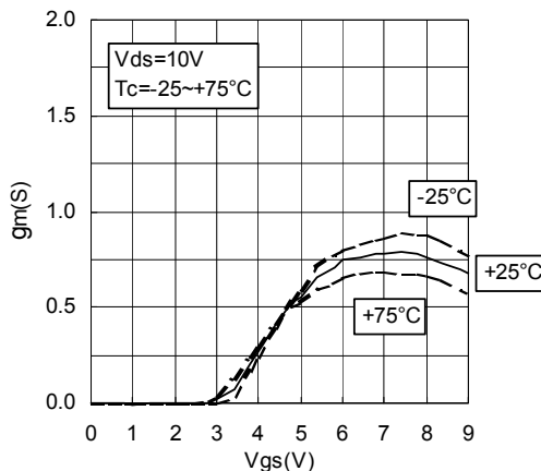
Vgs-gm CHARACTERISTICS
