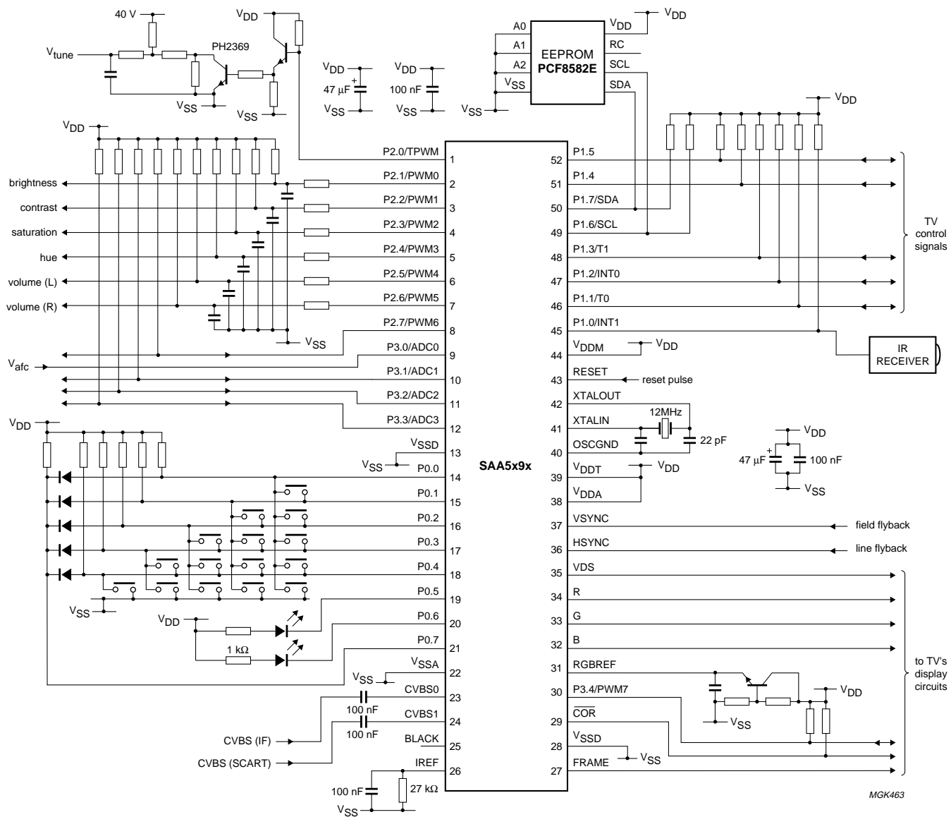
Fig.29 Application diagram.
