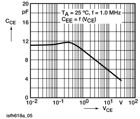
Fig. 8 - Transistor Capacitance
