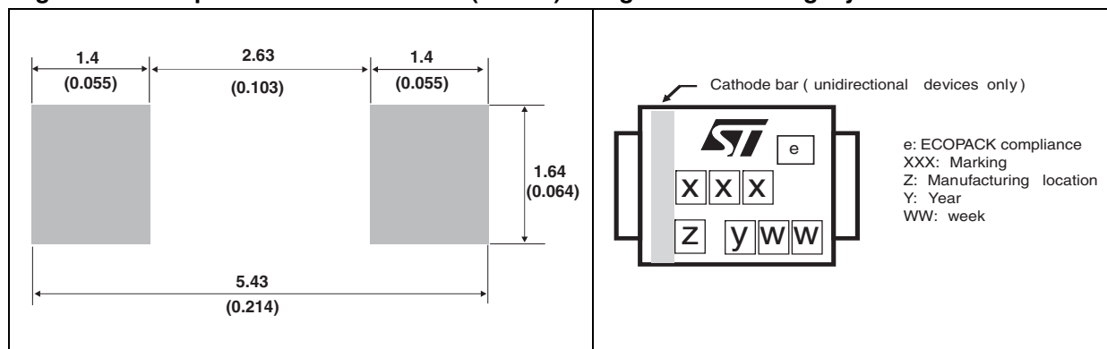
Figure 13. Footprint dimensions in mm (inches) Figure 14. Marking layout (1)
