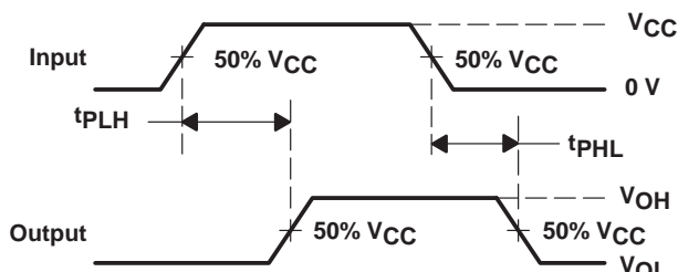
VOLTAGE WAVEFORMS
