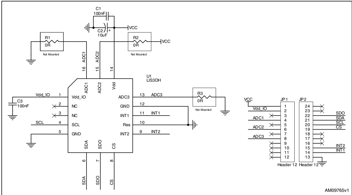
Figure 1. Circuit schematic
